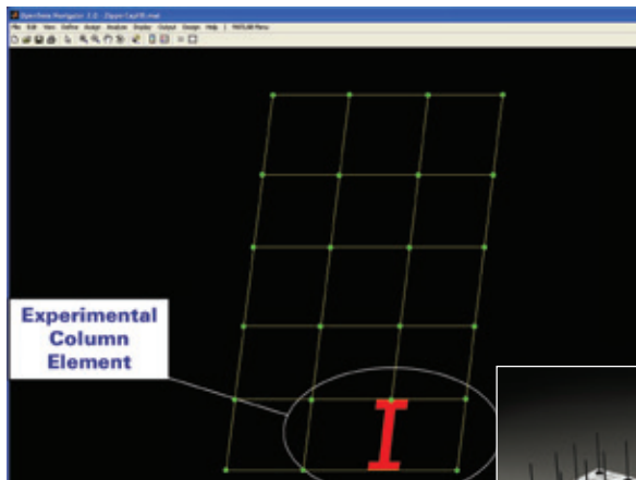
Representation of University of Colorado Boulder Hybrid Simulation Setup
