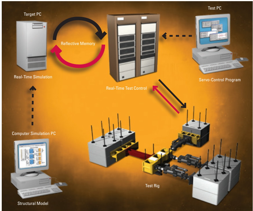
MTS Real-Time Hybrid Simulation
